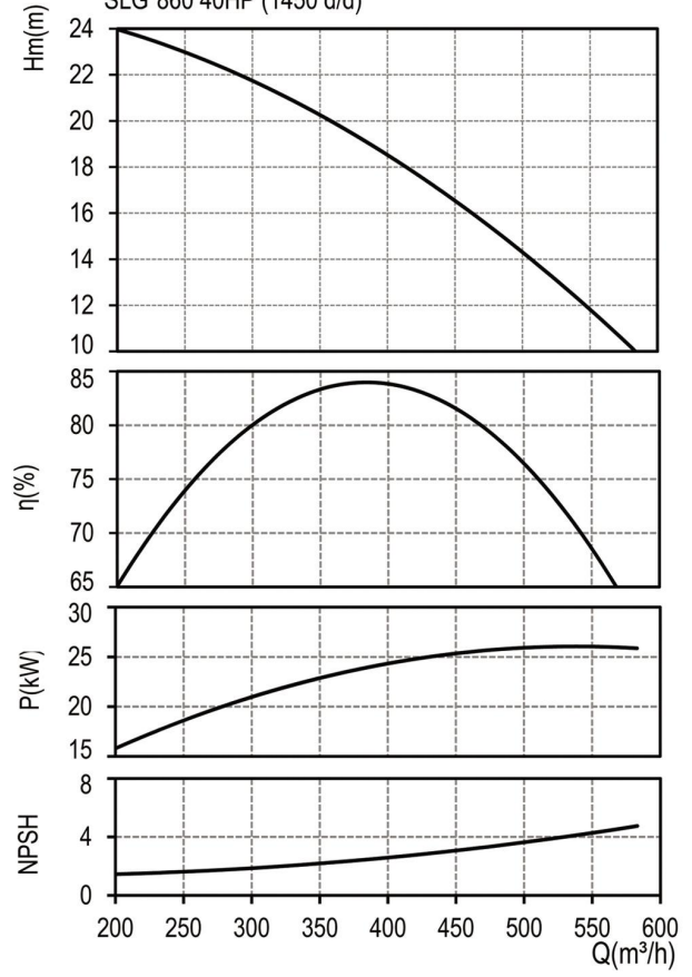
SLGM 860 40HP (1450 d/d) SLG 860 40HP (1450 d/d)
