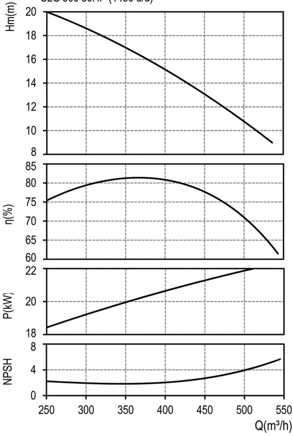
SLGM 860 30HP (1450 d/d) SLG 860 30HP (1450 d/d)
