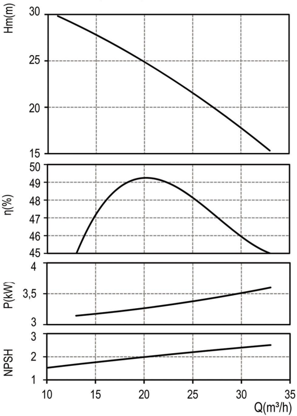
SLSD 2 4HP (2900 d/d)
