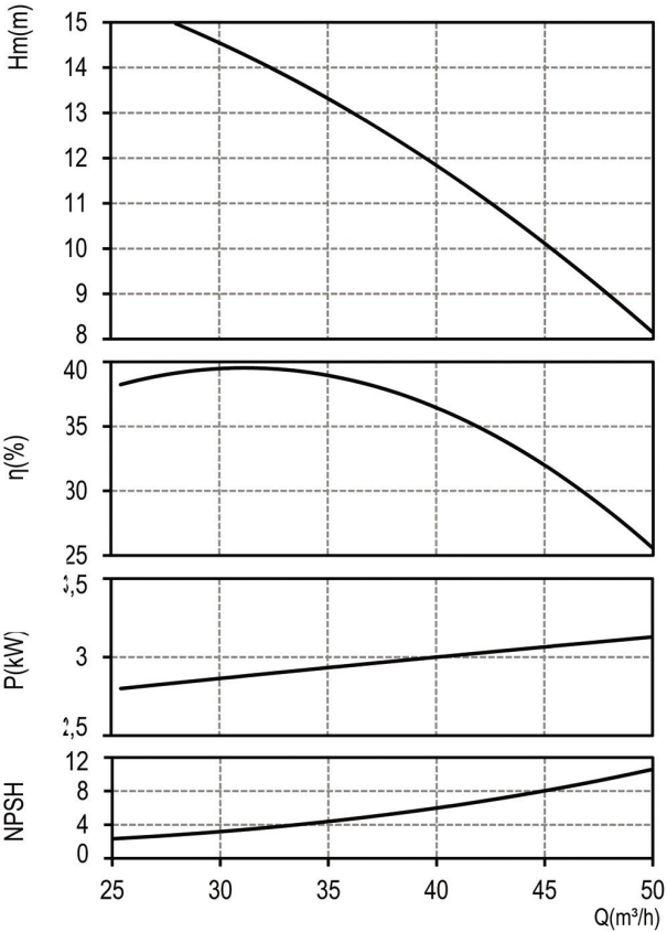
SD 430 4HP (1450 d/d)
