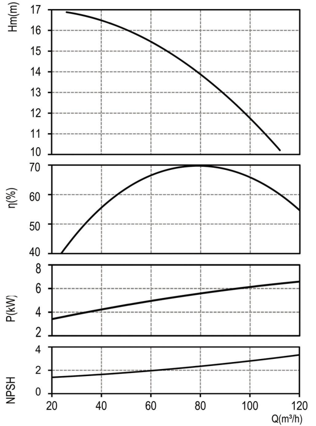
SD 540A 5,5HP (1450 d/d)
