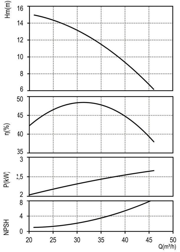
SD 430 3HP (1450 d/d)
