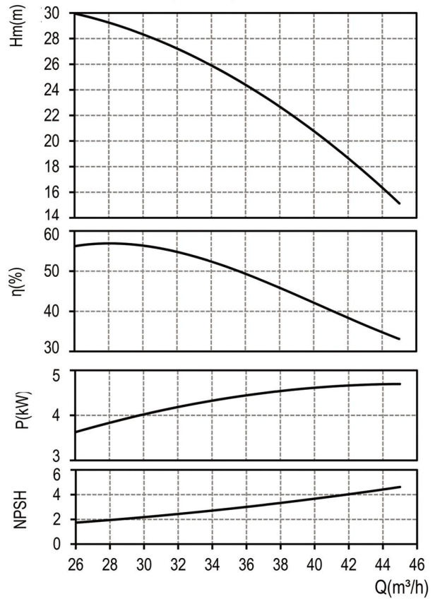
SLSD 2 5,5HP (2900 d/d)
