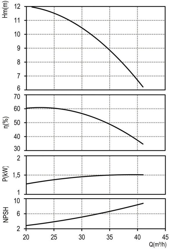
SD 325 2HP (1450 d/d)
